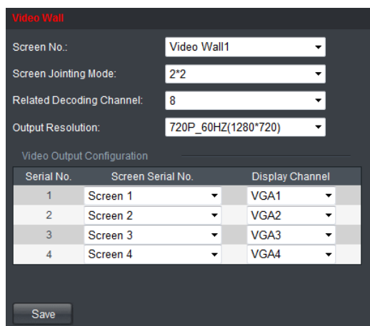
Figure 4.13 Configure Video Wall
