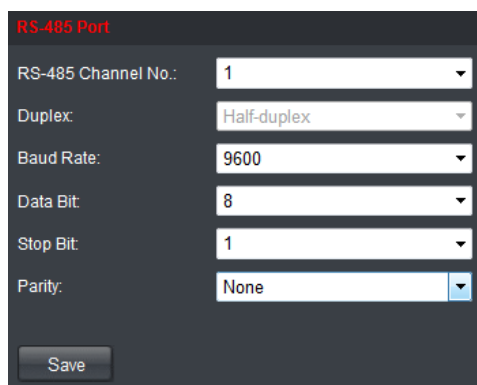
Figure 4.33 Configure RS-485 Settings
