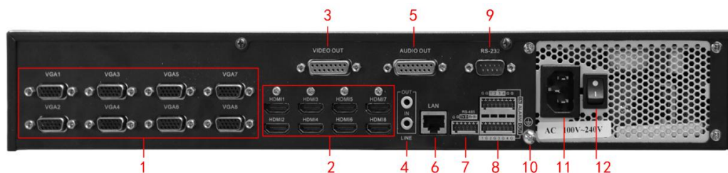
Figure 2.2 Rear Panel of DS-6408HDI-T
