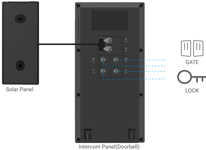
1-1 wiring diagram
