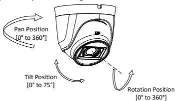
Figure 2-12 3-Axis Adjustment
