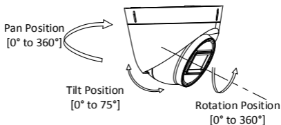
Figure 2-5 3-Axis Adjustment
