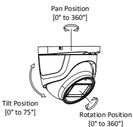
Figure 2-20 3-Aixs Adjustment
