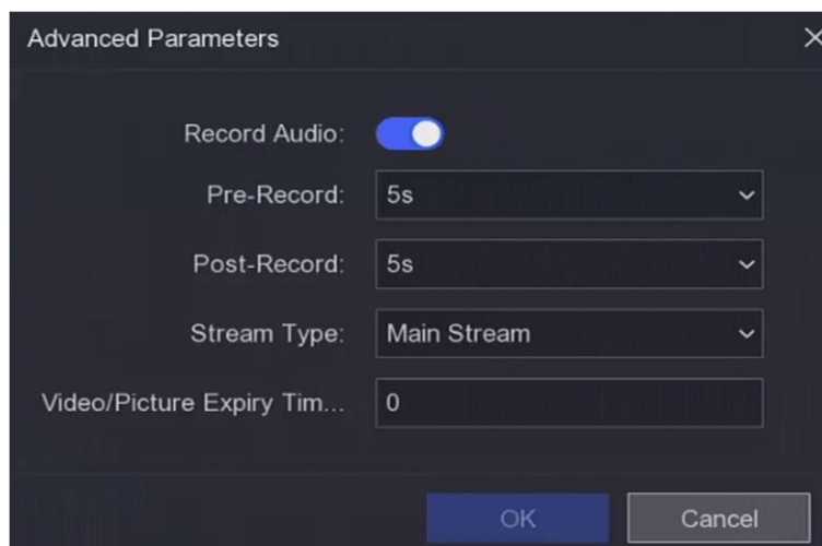
Figure 6-26 Advanced Parameters
