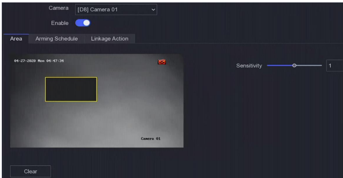
Figure 6-15 Video Tampering
