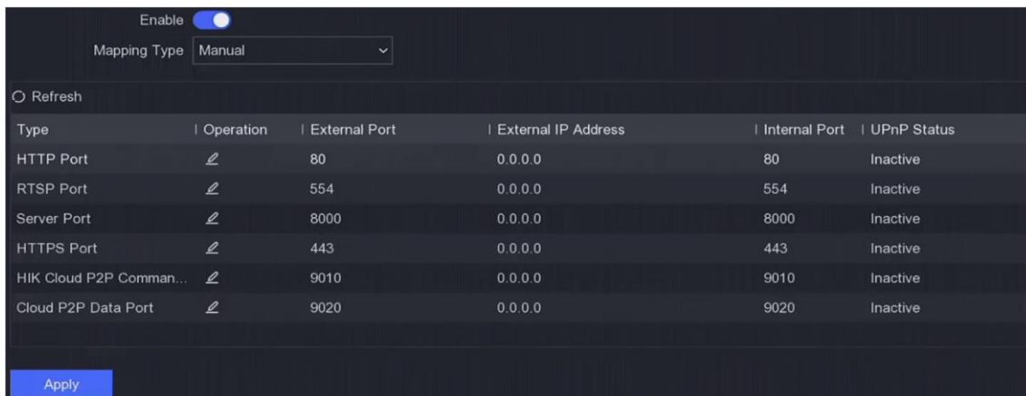
Figure 6-5 NAT
