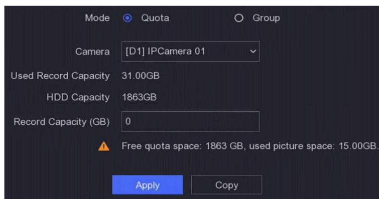
Figure 6-29 Quota
