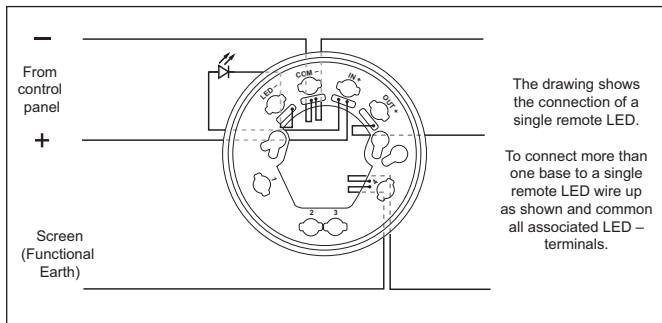
Fig 2 Wiring diagram
