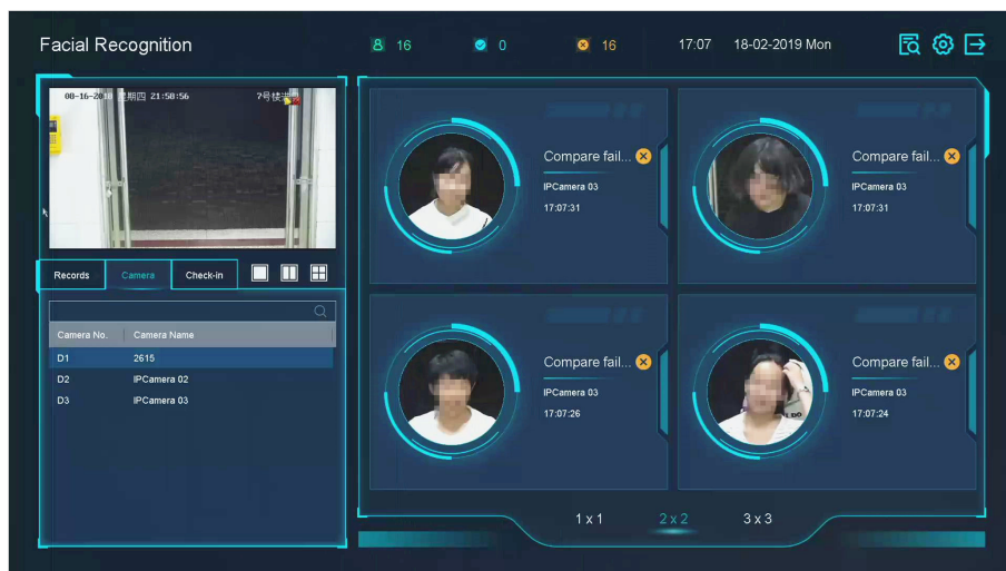
Figure 3-5 Facial Recognition
