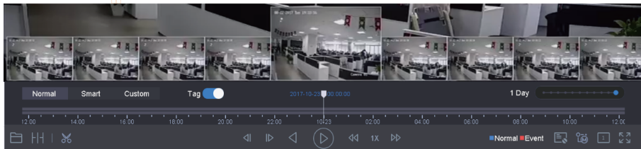
Figure 4-13 Thumbnails View
