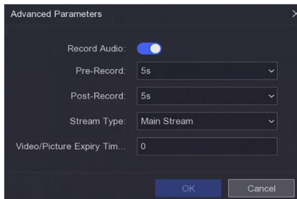
Figure 6-23 Advanced Parameters
