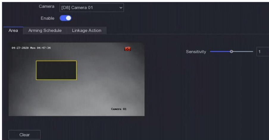
Figure 6-14 Video Tampering
