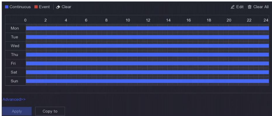
Figure 6-22 Recording Schedule
