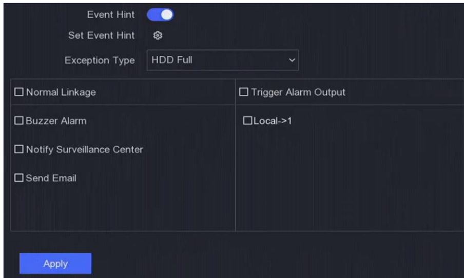
Figure 6-19 Exceptions
