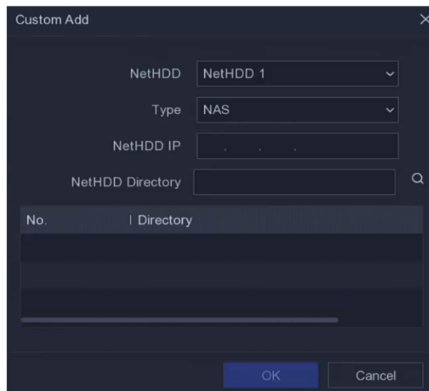
Figure 6-24 Add NetHDD
