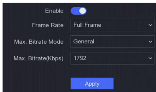
Figure 6-4 Channel-Zero
