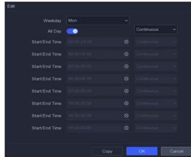
Figure 5-18 Edit Schedule
