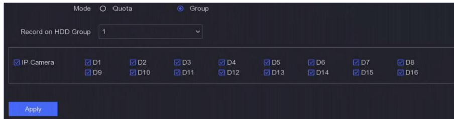
Figure 6-25 Group
