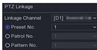
Figure 6-21 PTZ Linkage
