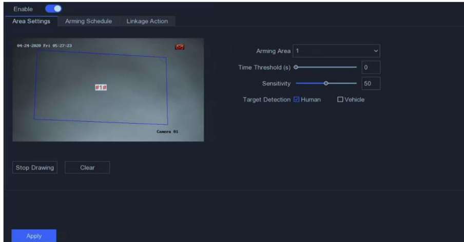
Figure 5-12 Intrusion Detection
