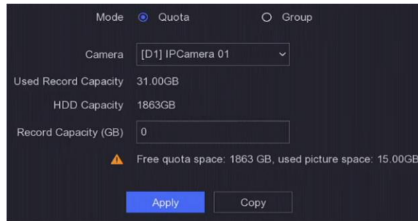
Figure 6-26 Quota
