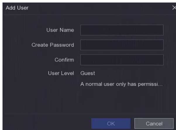
Figure 5-2 Add User
