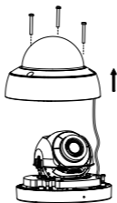
Figure 2-7 Remove the Bubble
