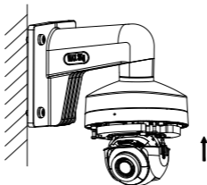
Figure 2-10 Install the Camera to the Bracket
