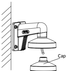
Figure 2-9 Install the Cap to the Bracket
