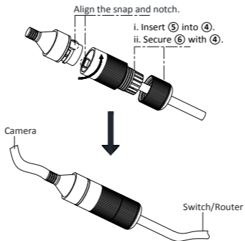
Figure 2-16 Waterproof Accessory Installation
