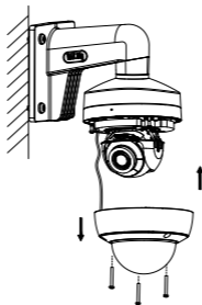
Figure 2-11 Install the Bubble to the Camera
