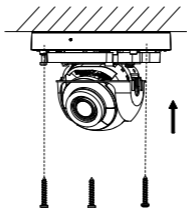
Figure 2-5 Secure the Camera
