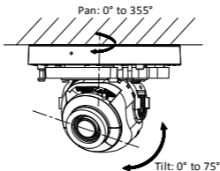
Figure 2-12 Angle Adjustment
