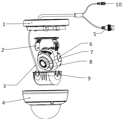
Figure 1-1 Overview of Camera
