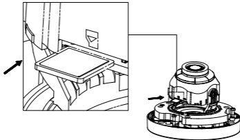
Figure 2-2 Remove the Bubble
