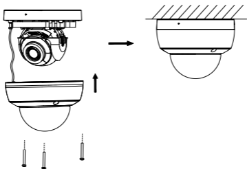
Figure 2-6 Secure Black Liner and Bubble
