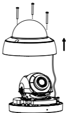
Figure 2-3 Remove the Bubble
