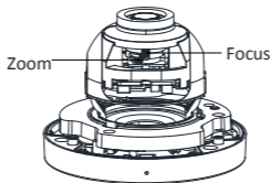
Figure 2-13 Zoom/Focus Lever
