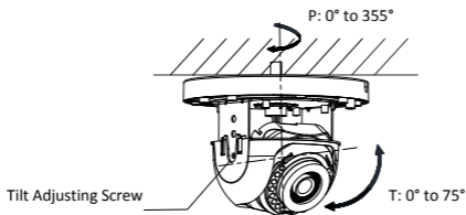
Figure 2-5 2-Axis Adjustment
