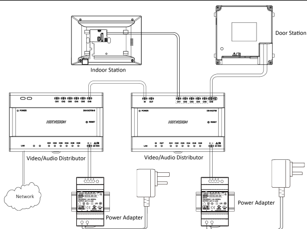
Figure 2-1 Wiring Description
