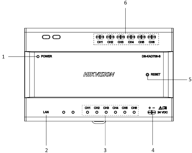
Figure 1-1 Video/Audio Distributor Appearance Table 1-1 Description
