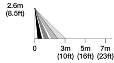
SIDE VIEW (Creep Zone)
